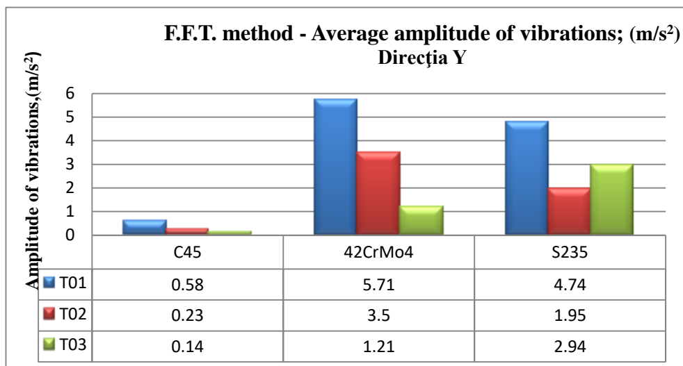
Figure 5.2. The results obtained by applying the F.F.T. method following the research of processing by turning with transverse advance a materials C45, 42CrMo4 and S235;
