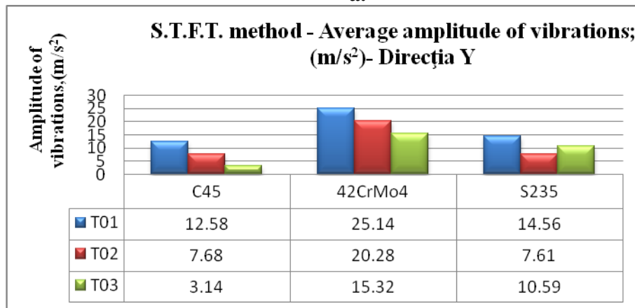
Figure 5.4 . The results obtained by applying the S.T.F.T. method following the research of processing by turning with transverse advance a materials C45, 42CrMo4 and S235;
